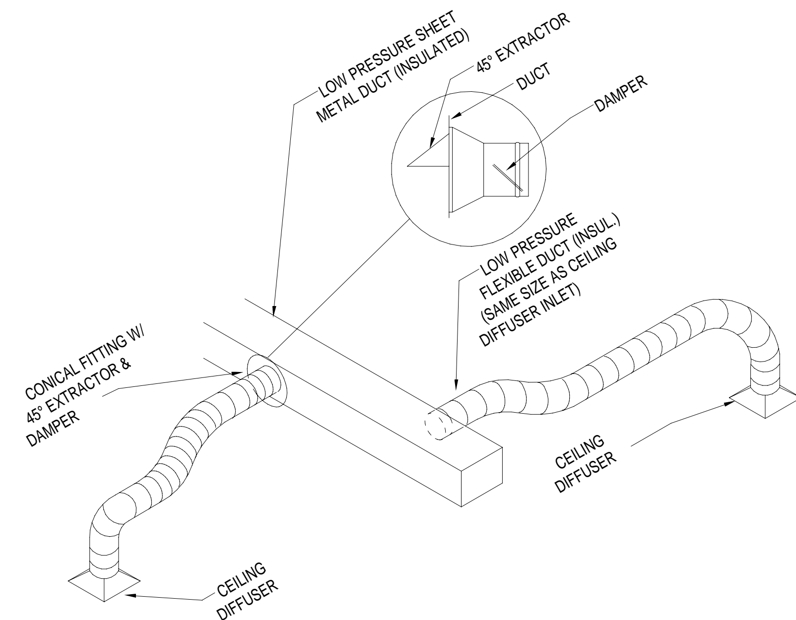
1 M102 DETAIL - DIFFUSER CONNECTION NOT TO SCALE
