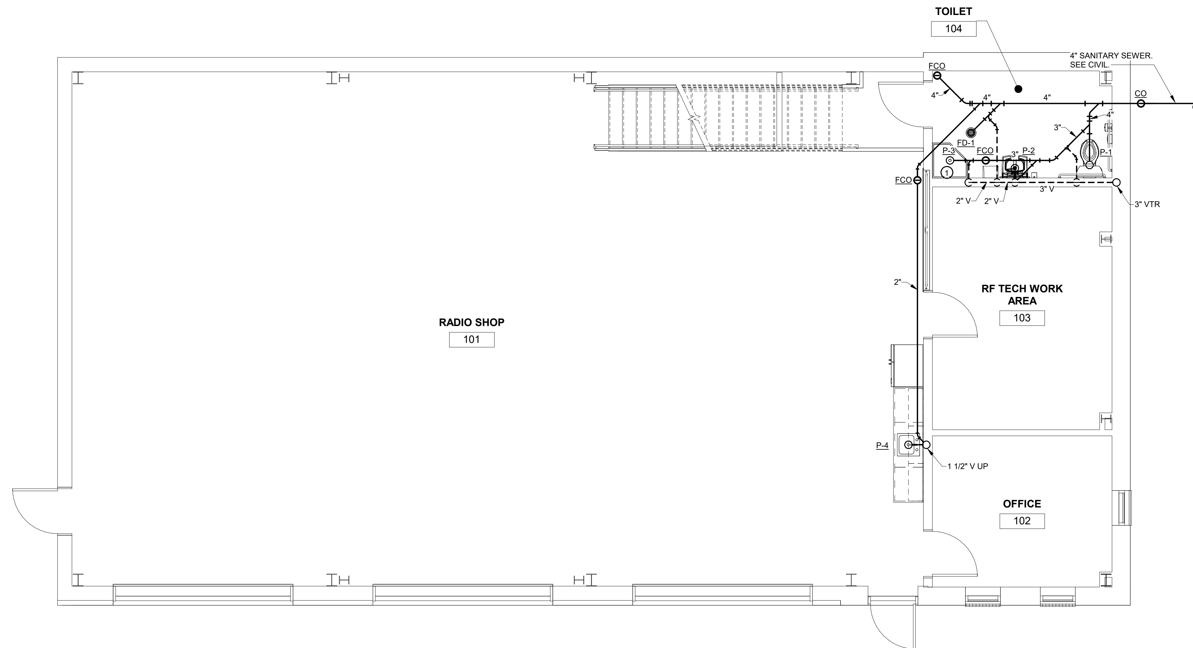
1 PLUMBING FIRST FLOOR SANITARY & VENT PLAN P3 1/4" = 1'-0"
