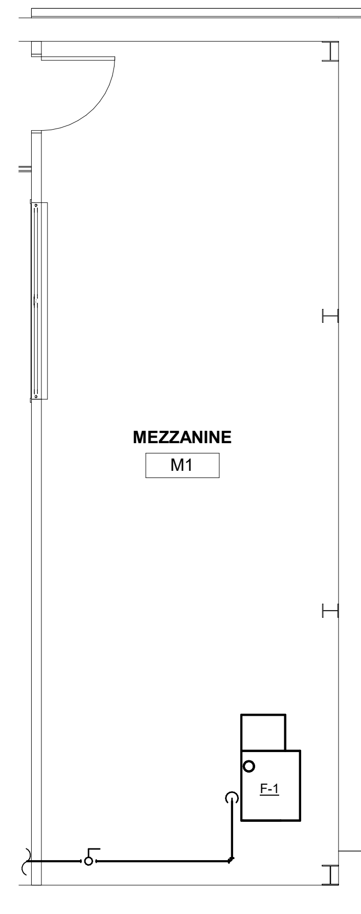
PLUMBING MEZZANINE NATURAL GAS PLAN 1/4" = 1'-0"
