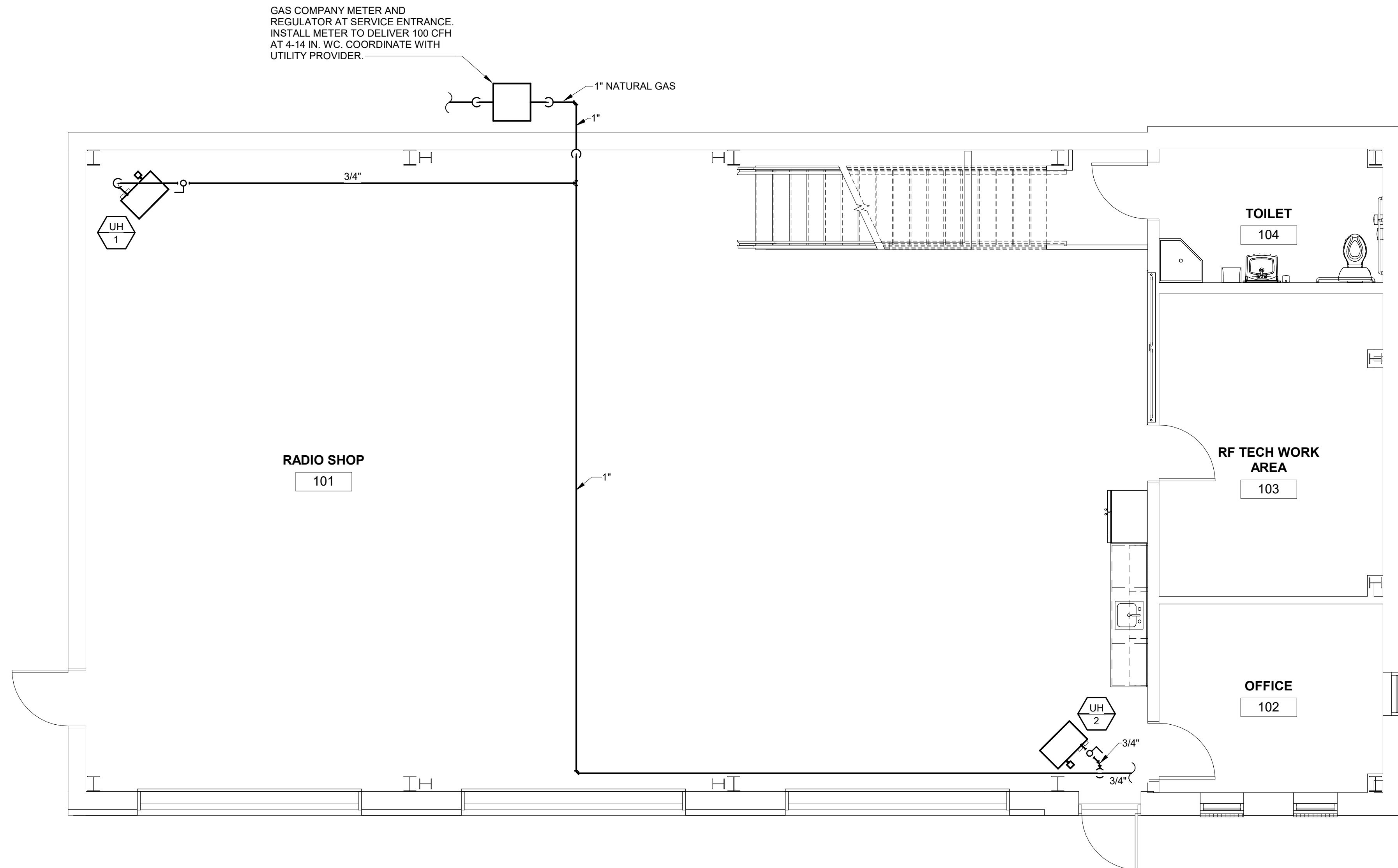
PLUMBING FIRST FLOOR NATURAL GAS PLAN 1/4" = 1'-0"
